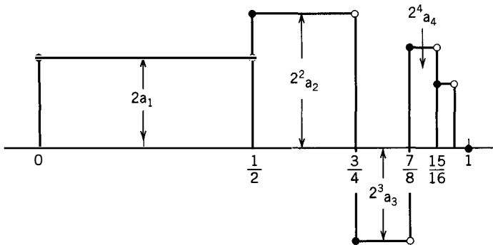
Figure 10.2.1 The graph of \varphi .
