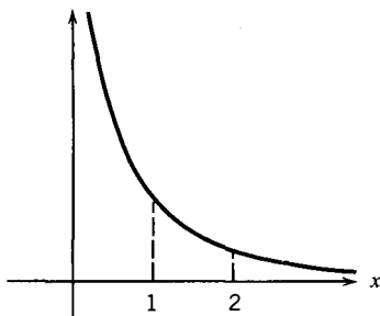
Figure 5.3.1 The function f(x) = 1/x ( x > 0 ).
