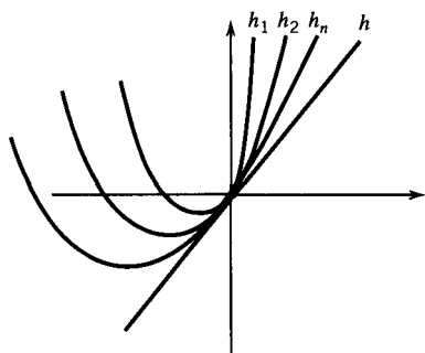
Figure 8.1.3 h_n(x) = (x^2 + nx)/n ,
