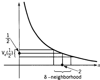
Figure 5.4.1 g(x) = 1/x \quad (x > 0) .
