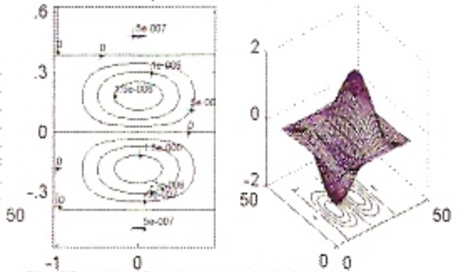
Fig.(26),paths of particales projected on the cross-section for \beta=0.044, k=1.77, L=0.01, \tau=1.753
