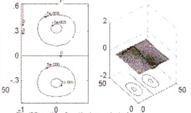
Fig.(30),paths of particales projected on the cross-section for \beta=0.044, k=1.77, L=0.01, \tau=2.6
