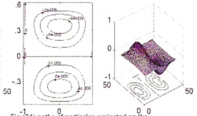
Fig.(24),paths of particales projected on the cross-section for \beta=1, k=1.77, L=0.01, \tau=2.2
