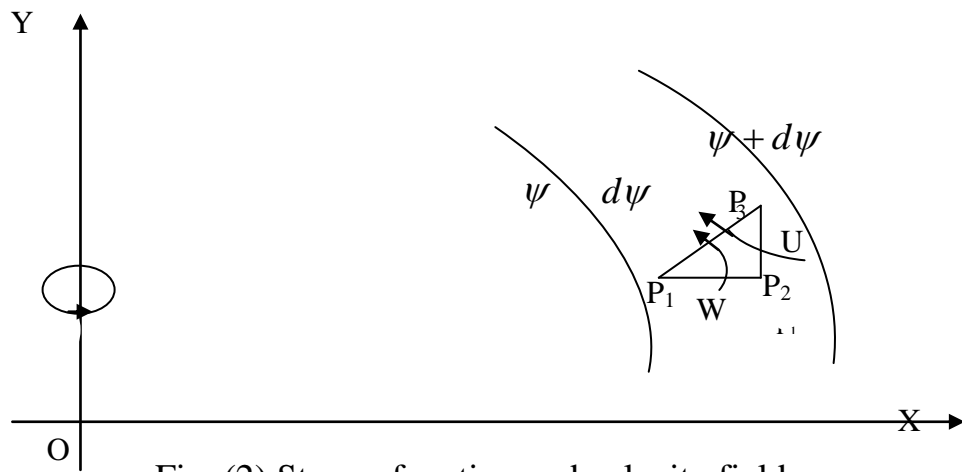
Fig. (2), Stream function and velocity field
