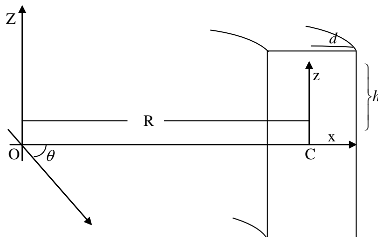
Fig.(6), Coordinates system
