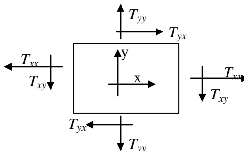
Fig.(3),Normal and Tangential Stresses
